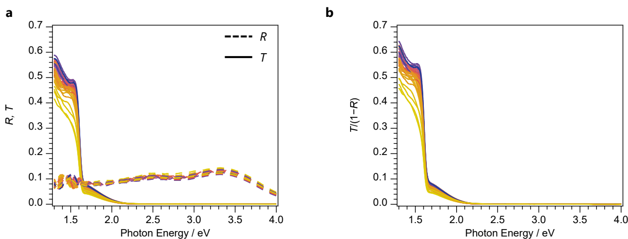
Figure S 2. a) Measured reflectance and transmittance of a combinatorial library, showing interference fringes around the bandgap of approx. 1.6 eV. b) Resulting reflection corrected transmittance.
