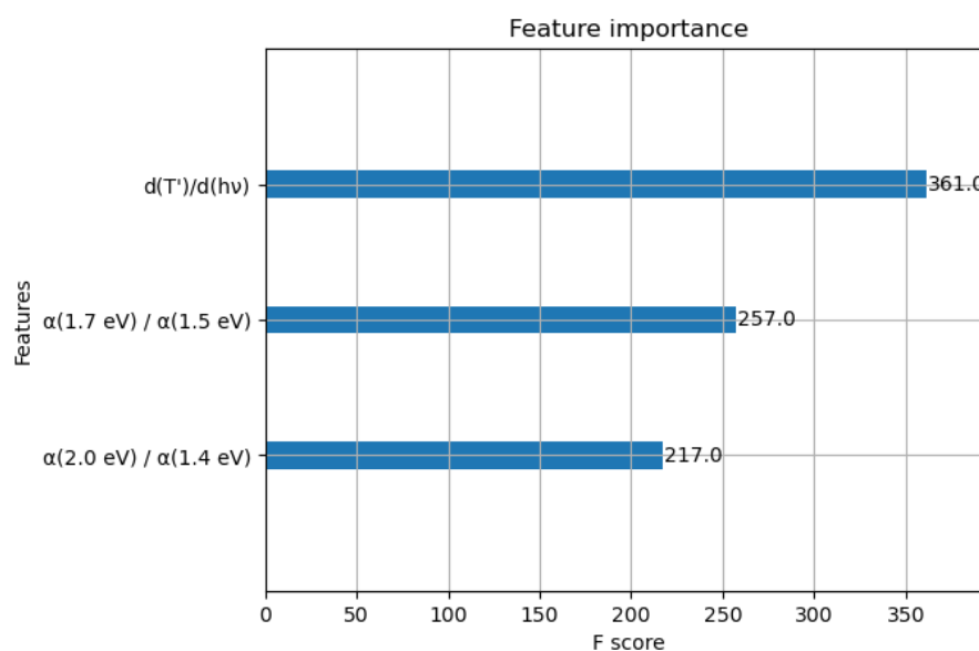
Figure S 11. Feature importance of the optimized XGBRegressor model.
