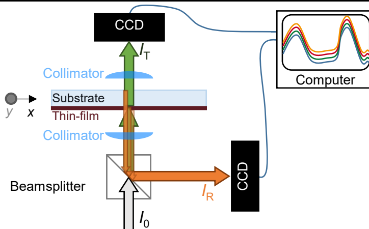
Figure S 1. Schematic of the beam path and position of the beam splitter and collimators. The light intensity of the light source I_0 is attenuated through the sample transmission or reflection.
