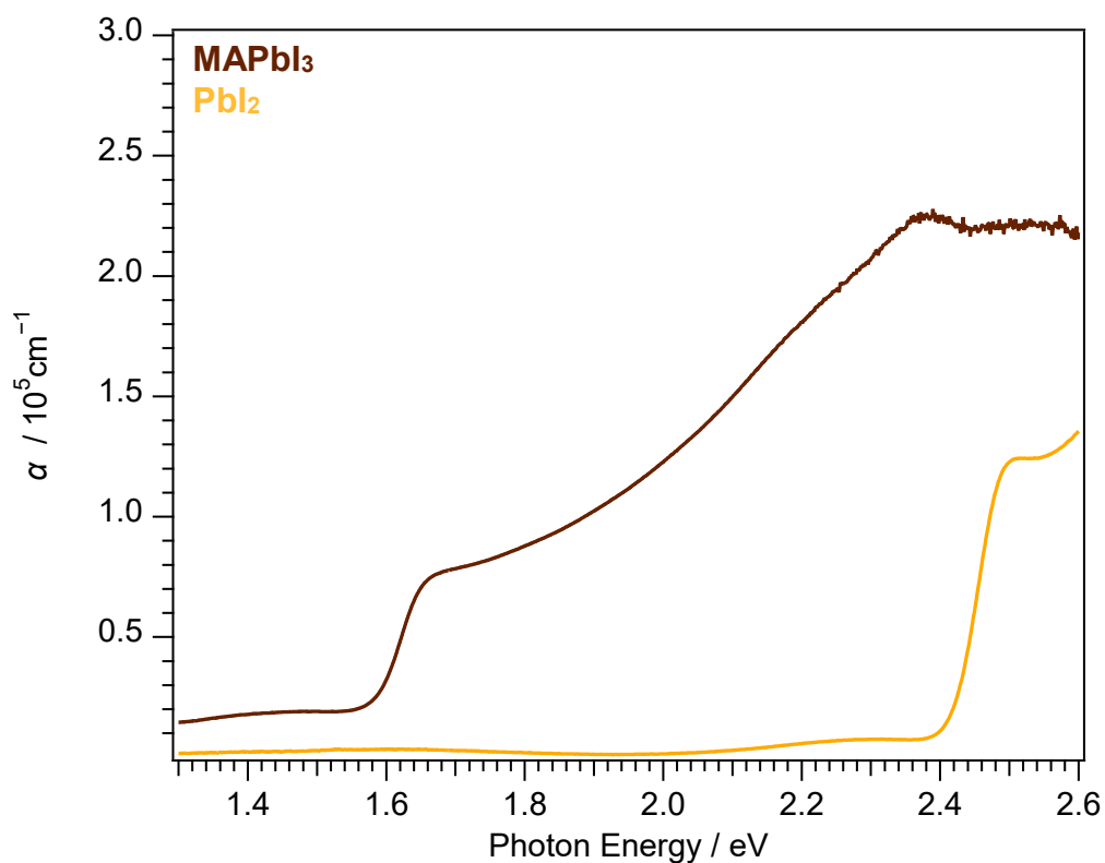
Figure S 9. Absorption coefficient \alpha vs Photon Energy for a thermally evaporated PbI 2 template and a resulting MAPbI 3 thin-film with a high conversion rate with band gaps of approx. 2.4 eV and 1.6 eV, respectively.
