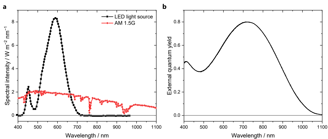
Figure S 3. A) Calibrated spectral intensity of the LED light source used against the AM 1.5G spectrum. B) Spectral external quantum yield (EQY) of the photodiode used to set the light intensity of the LED light source.
