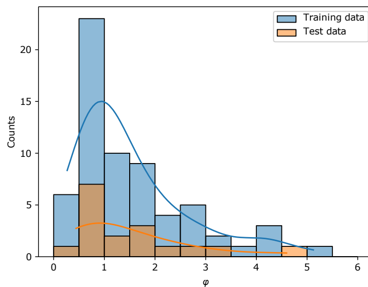
Figure S 13. Distribution of MHP/PbI 2 phase ratio within the training and test data expressed as a histogram with an overlaid probability distribution function. Samples with a MHP/PbI 2 phase ratio of \phi > 2.5 constitute the minority, amounting to only 20% of the total training data. The distribution function exhibits a similar shape for both data sets, indicating a likewise representation of the biased distribution within both the training and test data.
