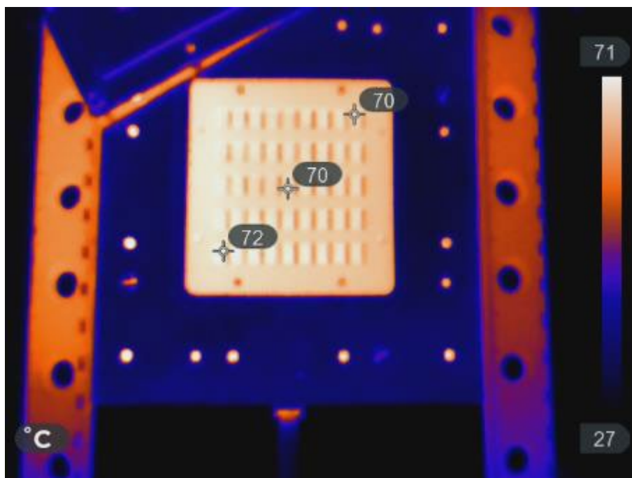
Figure S 5. False-colour thermal image of climate chamber with marked temperatures across the combinatorial grid, showing a standard deviation of <1^{\circ}\text{C} on perovskite thin-film library. An offset from the actual temperature of 85^{\circ}\text{C} resulted from the low emissivity of the samples on the substrate.
