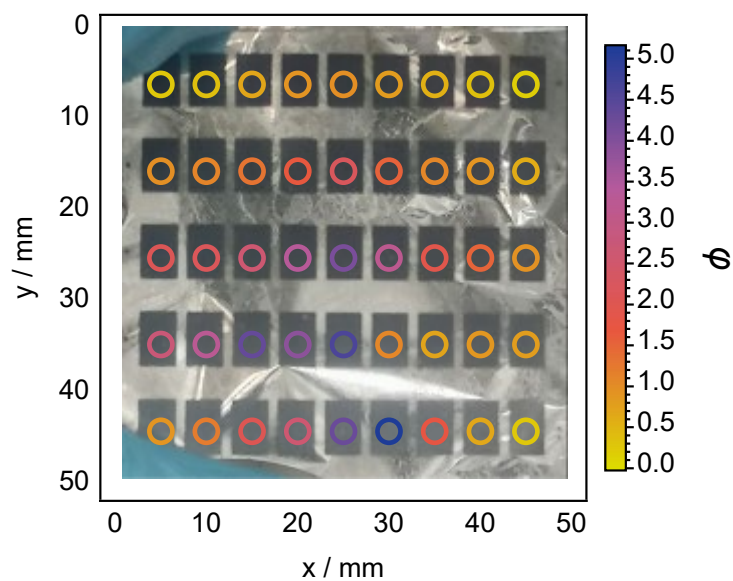
Figure S 8. Overlaid mapping of the MHP/PbI 2 phase ratio on top of a photograph of the pristine library. Behind the patterned library on the transparent substrate, an aluminum foil can be seen.
