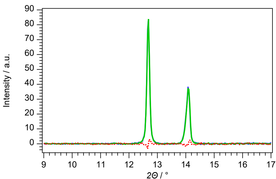
Figure S 7. XRD diffractogram of library samples measured within the inert-gas XRD Dome before (blue lines) and after (green lines) 17 h within the Dome. No significant change of the peaks was observed based on the differential spectrum (red dots).
