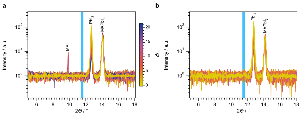
Figure S 6. 2\theta XRD measurements at shallower angles performed a) before and b) after the aging procedure. One sample exhibited a feature at approx. 9.8^\circ , indicative of residual unreacted MAI on the thin-film 1 which was however absent in the aged thin-films. Overconverted perovskite thin-films ( i.e. those with overstoichiometric amounts of A-site cations) can typically be detected at these shallower diffraction angles. 2,3 However, no similar feature could be detected at the angle previously reported for overconverted \text{MAPbI}_3 thin-films (blue marker). 1
