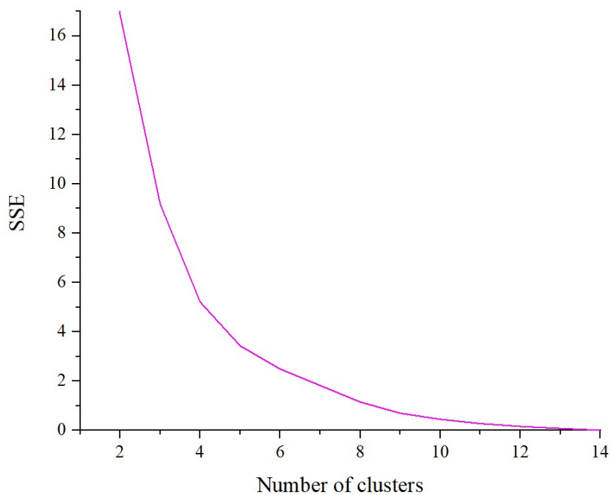
Figure S1. Dynamics of the sum of the squared error (SSE) reduction with increasing number of clusters
