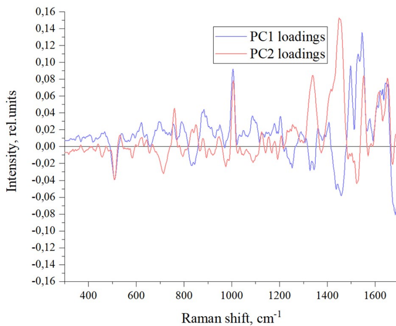
Figure S2. Loadings for PC1 and PC2 (for the PCA in Figure 2)
