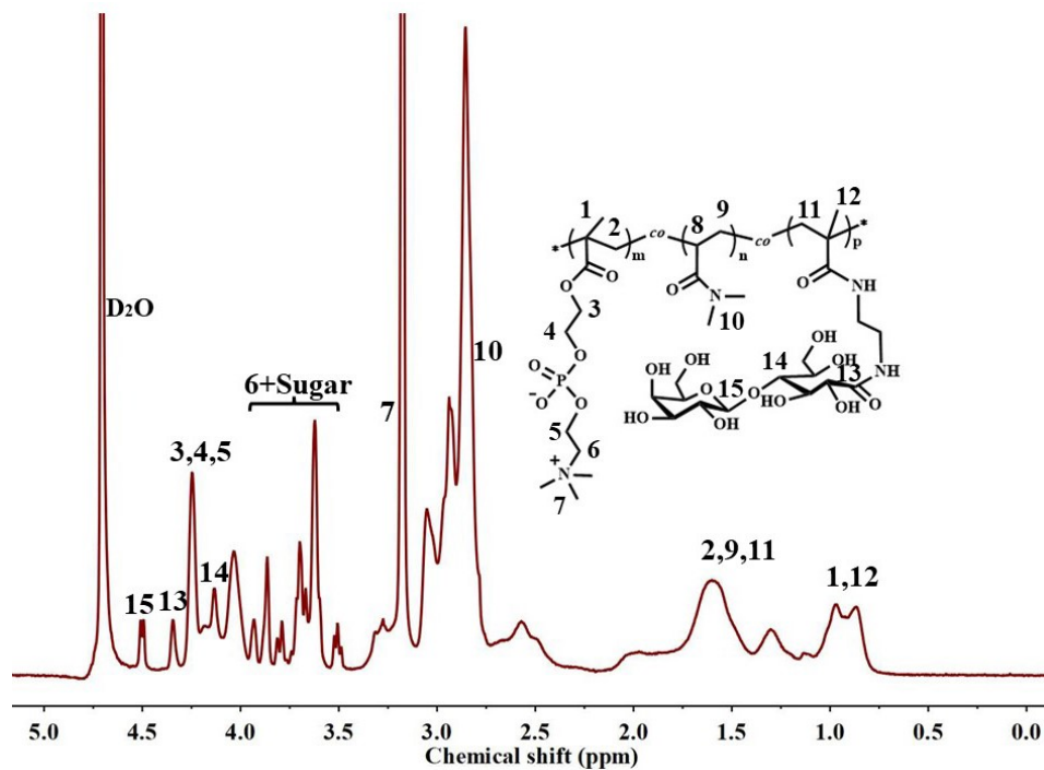
Figure S2. ^1\text{H} NMR spectrum of copolymer PMDL.
