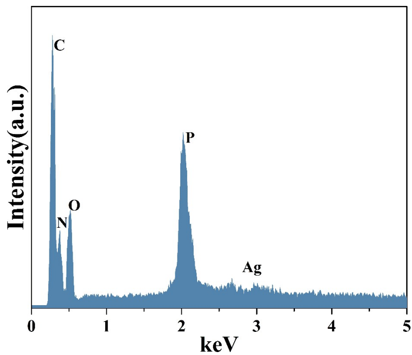
Figure S3. EDS spectrum of PMDL-12%/Borax/Ag NPs hydrogel
