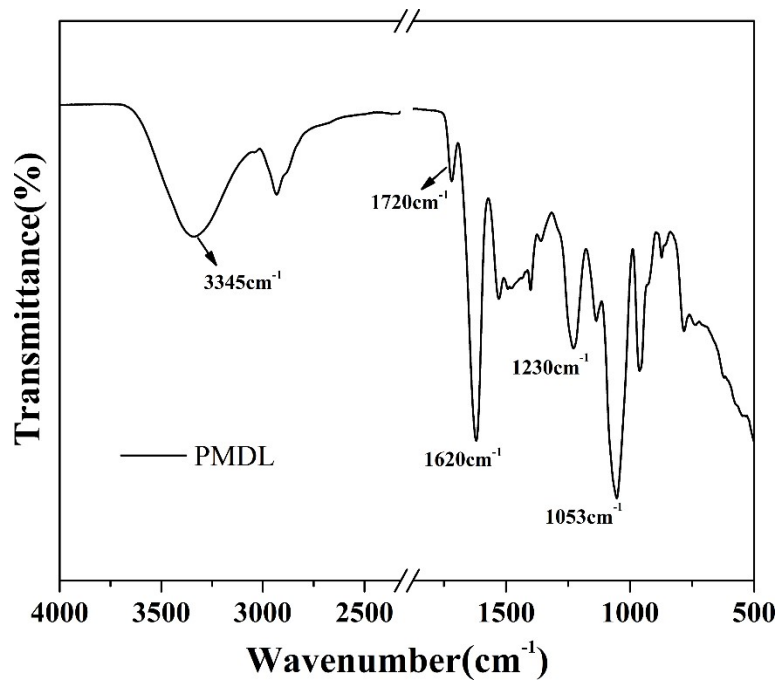
Figure S1. IR spectrum of poly[(2-methacryloyloxyethyl phosphorylcholine)- co -(N, N-dimethylacrylamide)- co -(2-lactobionamidoethyl methacrylamide)] (PMDL).
