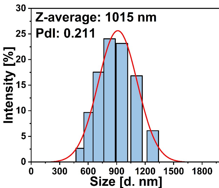
Fig. S1. The DLS measurement representing the PDA particle distribution, average size, and PDI.
