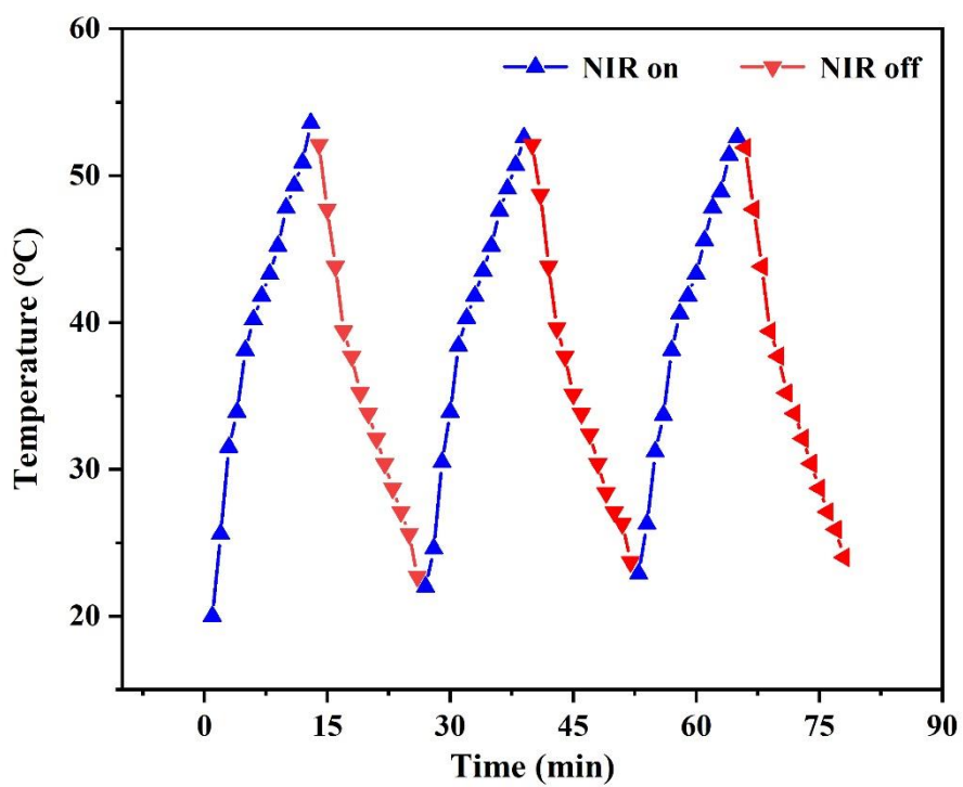
Fig.S1. The recycling heating profile of ATB hydrogel under NIR light irradiation ( 1 \text{ W}\cdot\text{cm}^{-2} ) for three on/off cycles.
