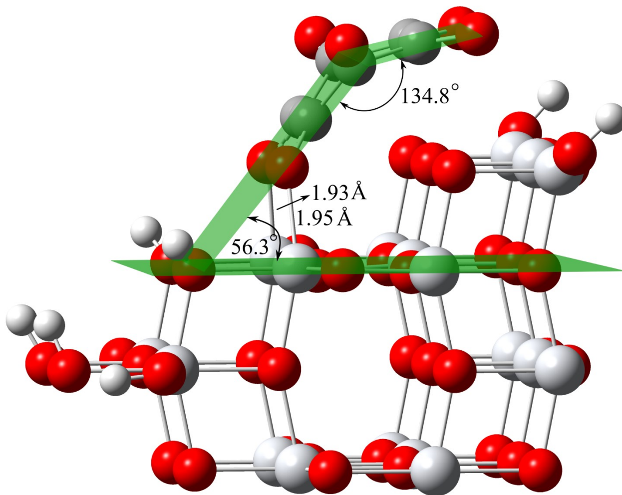
Supporting Information 3. Optimized geometry of the [\text{Ti}_{18}\text{O}_{31}(\text{OH})_8]/\text{RhA} cluster.
