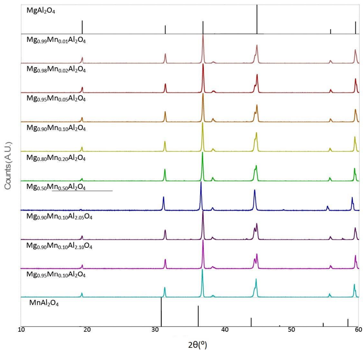
Figure S1 XRD on the top and bottom \text{MgAl}_2\text{O}_4 and \text{MnAl}_2\text{O}_4 reference spectrum are shown
