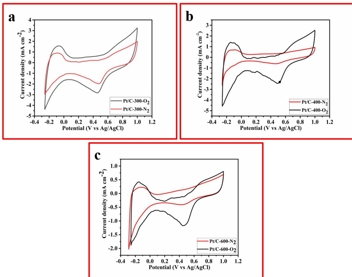
Figure S1. CV curves of (a) Pt/C-300, (b) Pt/C-400, and (c) Pt/C-600 in N 2 -saturated and O 2 -saturated 0.5 M H 2 SO 4 solution with a sweep rate of 50 mV s -1 .
