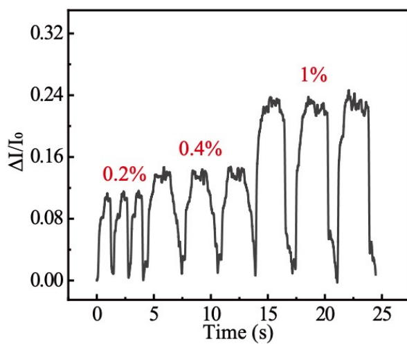
Figure S2. The minimum detection limit of the KFSS-60
