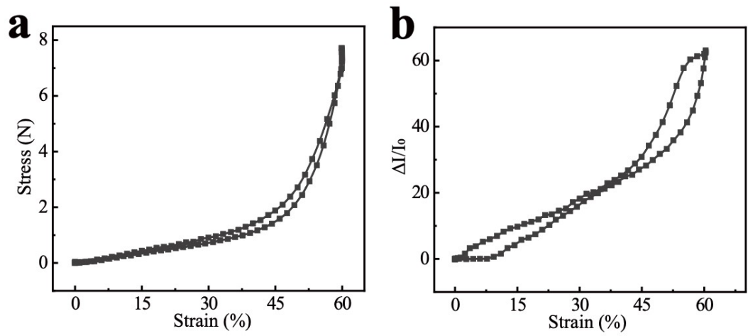
Figure S3. The mechanical and electrical hysteresis curves of the KFSS-60
