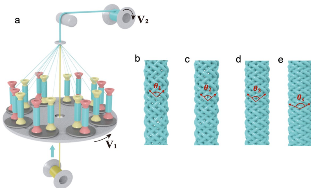
Figure S1. The illustration of the adjustment to the stretchability of the BSY
