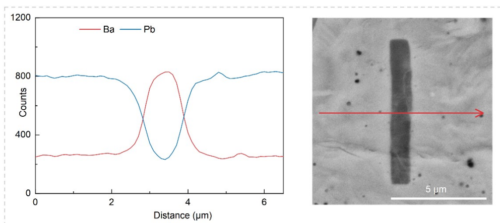
Fig. S2. EDS line scan across a BT template in BS-60PT-2BT matrix and the right shows corresponding SEM image.
