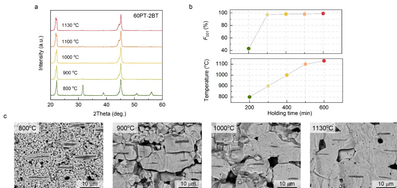
Fig. S1. (a) XRD patterns of BS-60PT-2BT ceramics with different sintering temperatures; (b) The variation trend of texture degree with sintering temperature; (c) SEM images of textured ceramics at different sintering temperatures.
