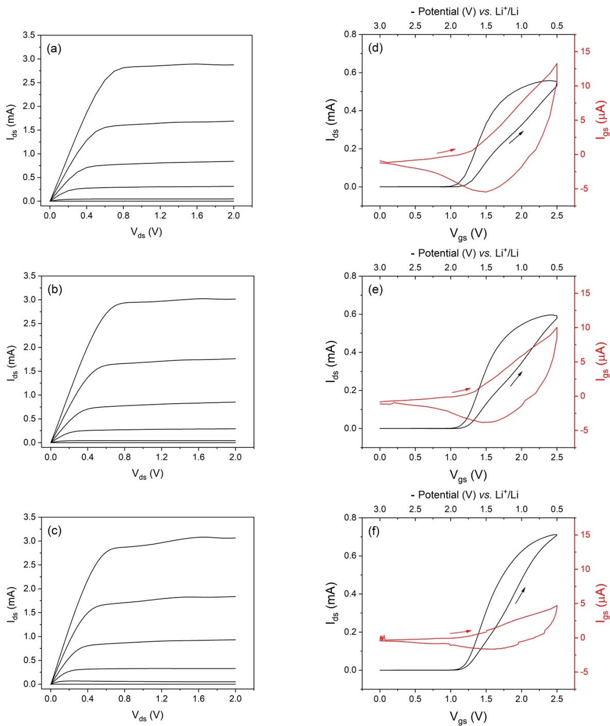
Fig. S6 \text{TiO}_2 IGTs without \text{Li}^+ in [\text{EMIM}][\text{TFSI}] . Output characteristics at V_{\text{ds}} sweeping rate of (a) 100 \text{ mV s}^{-1} , (b) 50 \text{ mV s}^{-1} , (c) 10 \text{ mV s}^{-1} , V_{\text{gs}} from 1 V to 2 V with 200 mV step. Transfer characteristics at 100 \text{ mV s}^{-1} , 50 \text{ mV s}^{-1} , 10 \text{ mV s}^{-1} (d, e, f), V_{\text{ds}}=100 \text{ mV} . Potential range 0 \text{ V} \leq V_{\text{gs}} \leq 2.5 \text{ V} .
