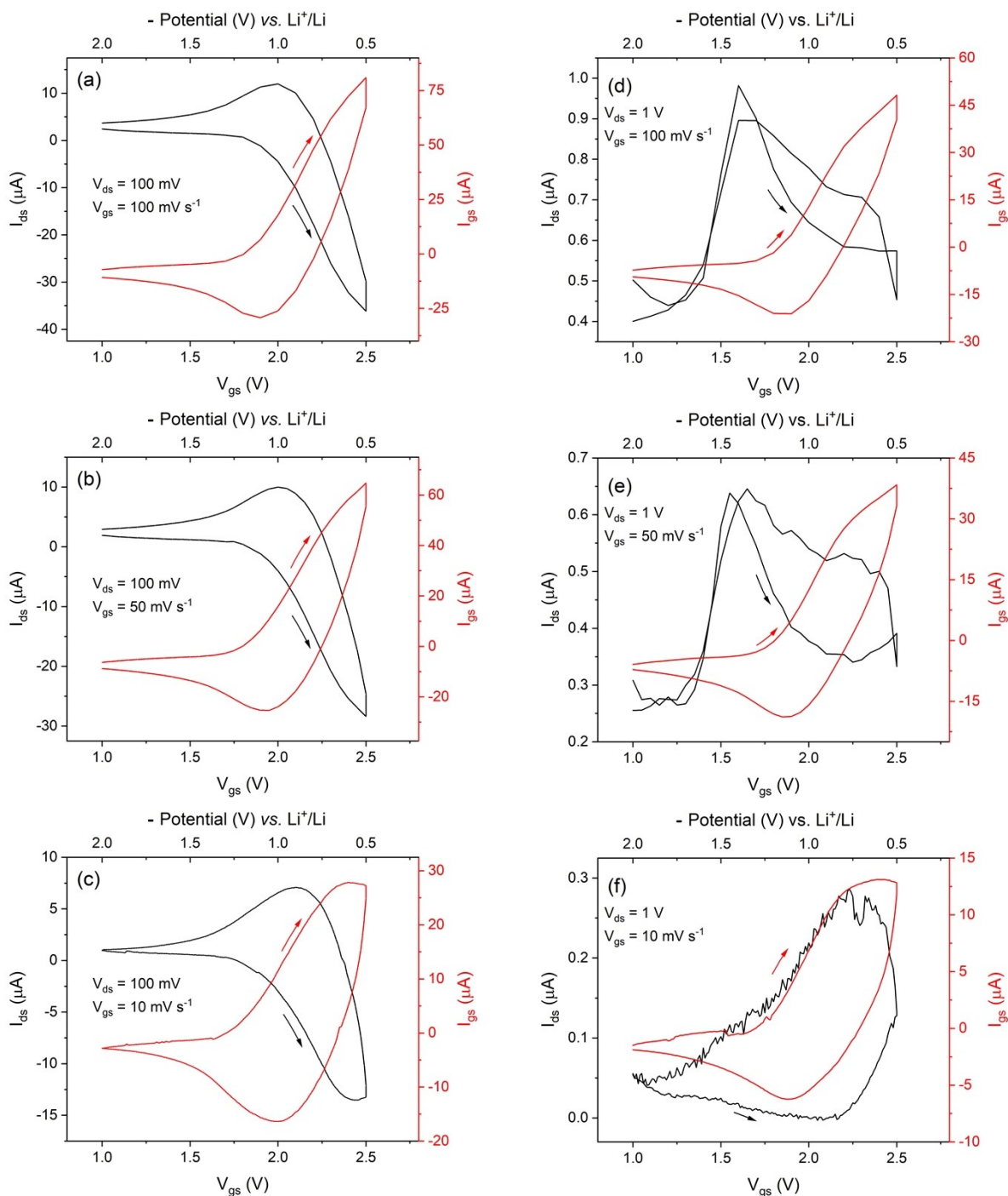
Fig. S4 Transfer characteristics of LTO with V_{ds} = 0.1 V at three V_{gs} sweeping rates, (a) 100, (b) 50, and (c) 10 \text{mV s}^{-1} . Additionally, with V_{ds}=1\text{V} and three V_{gs} sweeping rates (d) 100 \text{mV s}^{-1} , (e) 50 \text{mV s}^{-1} , (f) 10 \text{mV s}^{-1} . 0.1 \text{mol L}^{-1} LiTFSI in [EMIM][TFSI] as gating medium.
