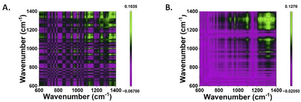
Figure S4: Two-dimensional correlation map in the range (600 – 1400 \text{cm}^{-1} ): (A.) Control (B.) Treated
