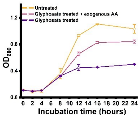
Figure S1: Growth curve of E. coli grown in M9 minimal medium, Glyphosate treated medium, Glyphosate treated medium supplemented with exogenous Aromatic Amino acids.
