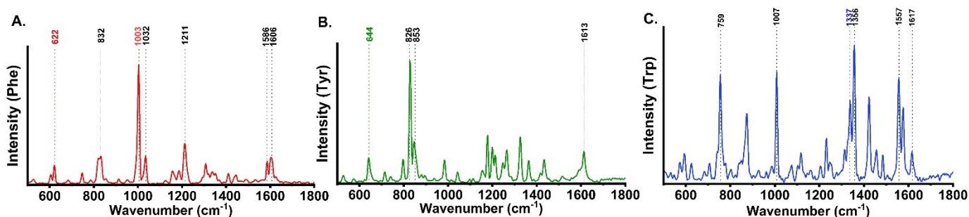
Figure S3: Mean Raman spectra of supplemented exogenous aromatic amino acid and the corresponding reference bands are marked in colours. (A) Phenylalanine (B) Tyrosine (C) Tryptophan.
