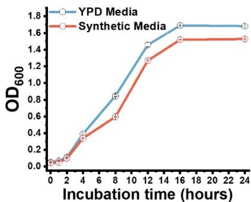
Figure S2: Evaluating the feasibility of Synthetic media with glucose as only carbon source for the growth of S. cerevisiae .
