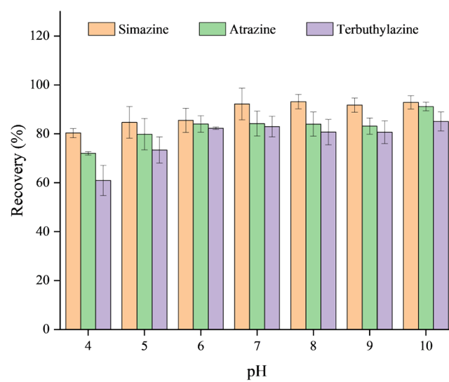
Fig. S2. Optimisation of pH.
