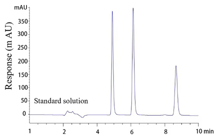
Fig. S1. Chromatograms of simazine, atrazine, and terbutylazine.
