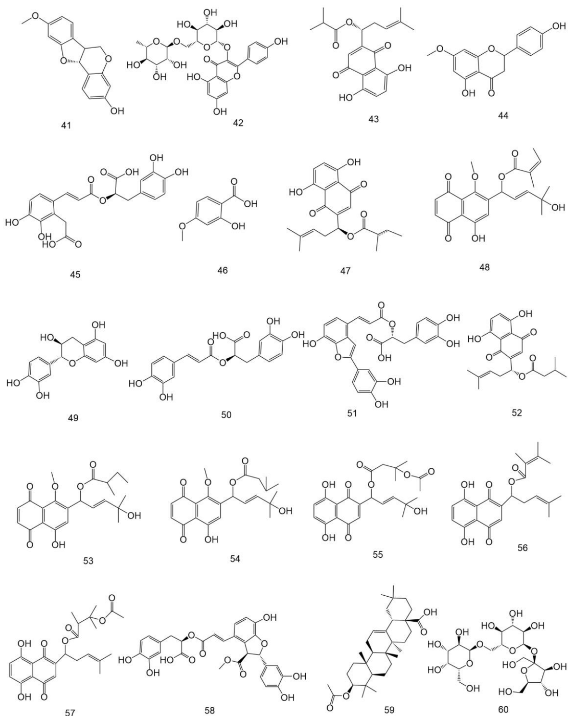
Structures of the identified compounds 41-60
