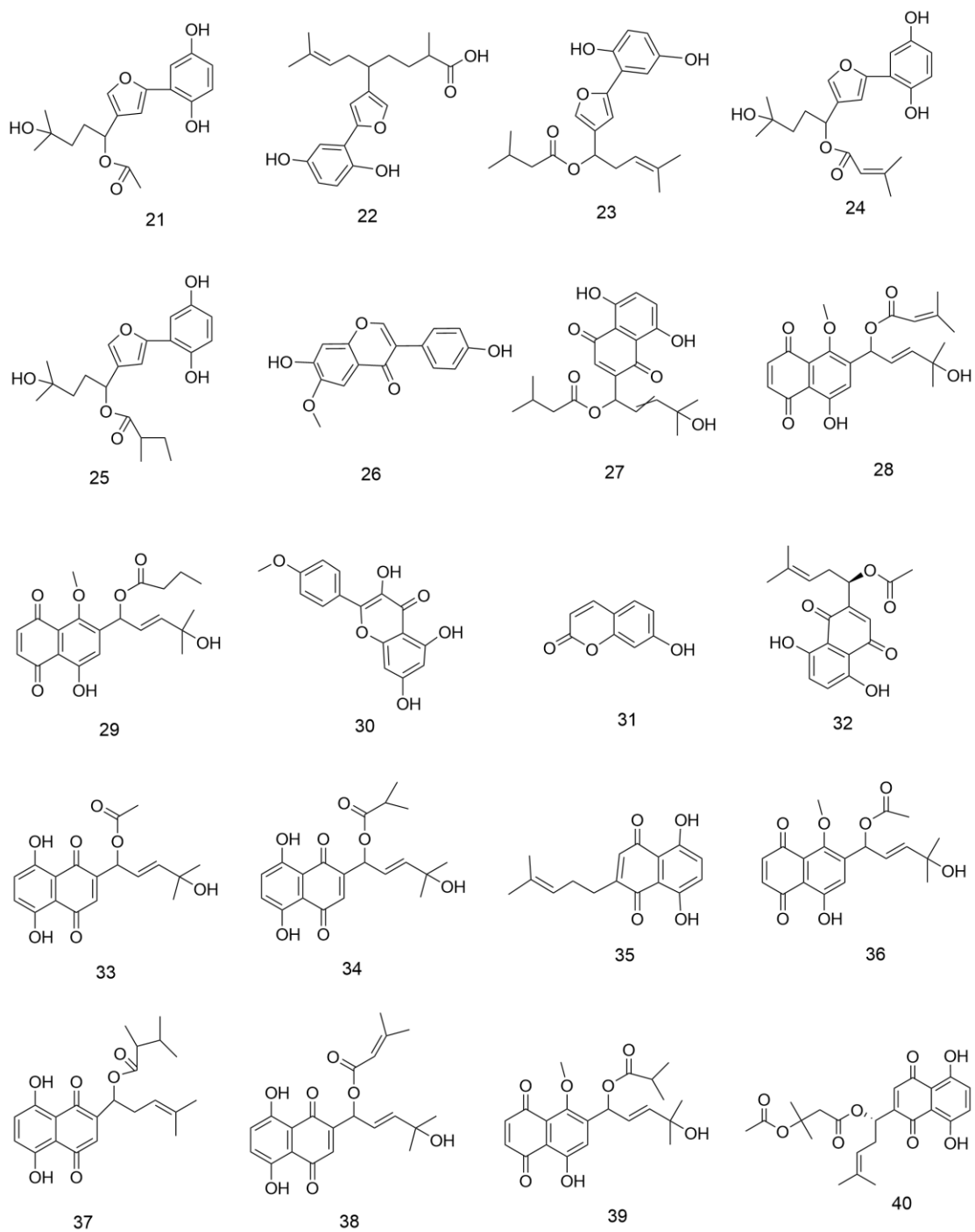
Structures of the identified compounds 21-40
