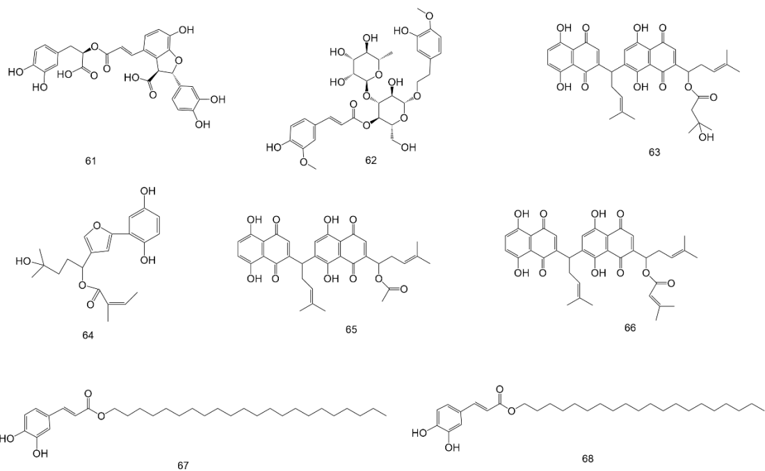
Structures of the identified compounds 61-68
