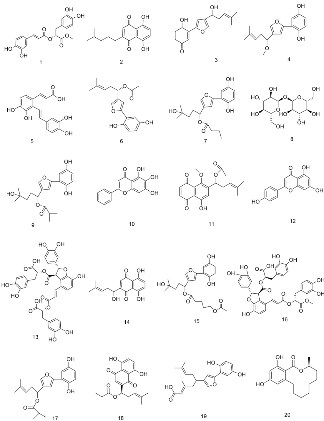
Structures of the identified compounds 1-20
