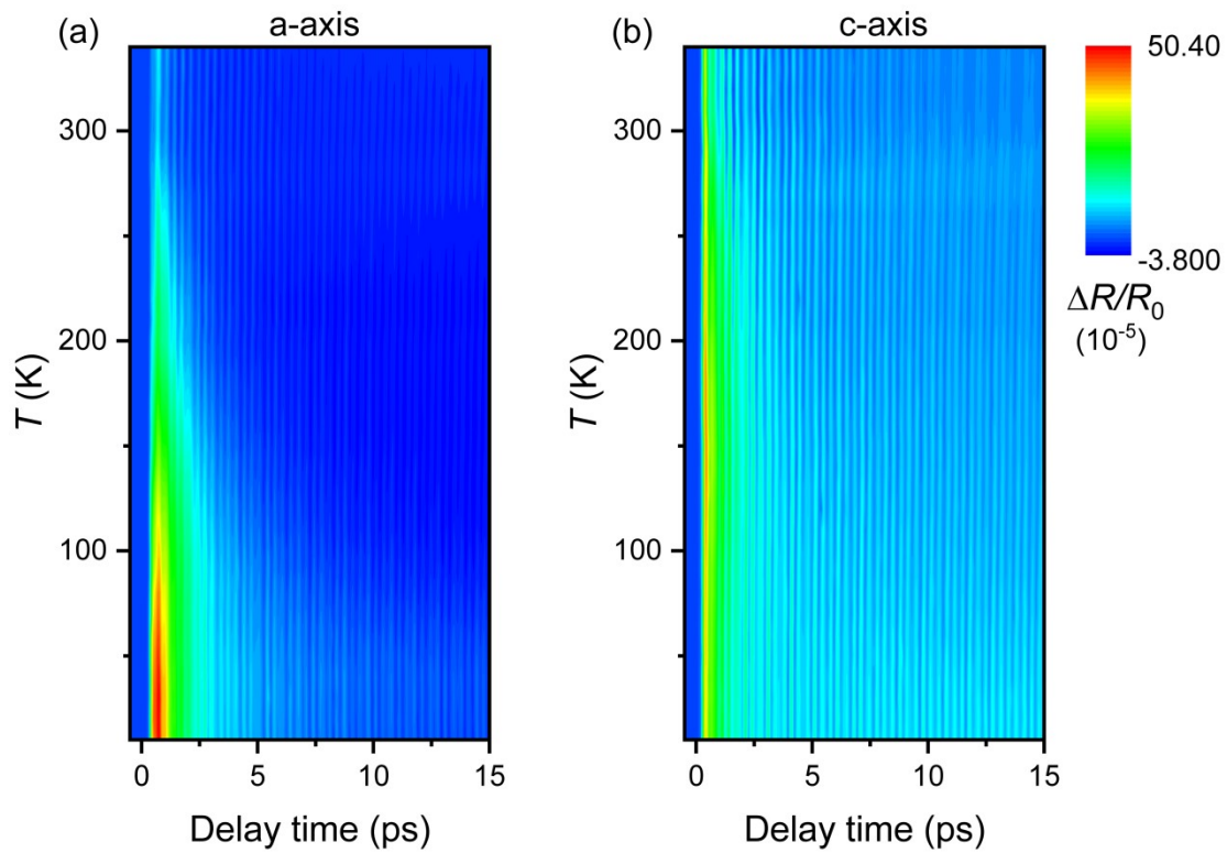
Fig. S1. Temperature-dependent \Delta R(t)/R_0 time series collected for a- and c-axis.
