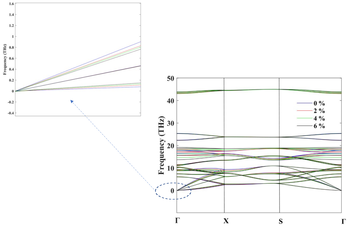
Figure S3: Phonon dispersion relation of penta-NiN2 at different applied strains calculated from DLP
