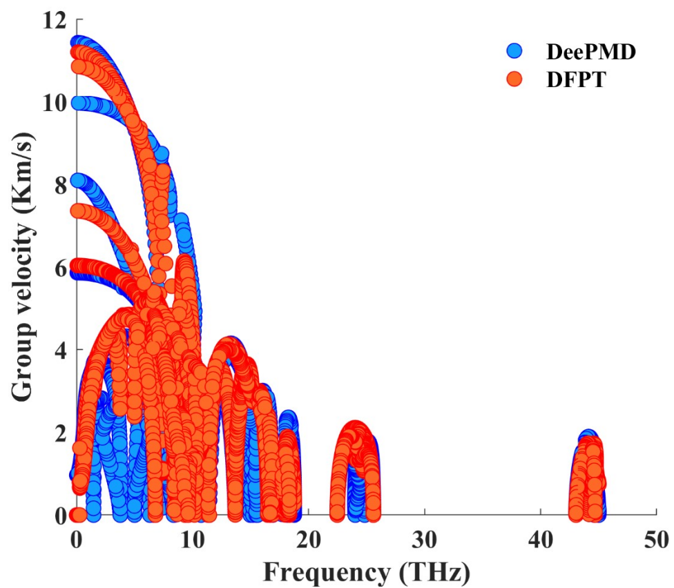
Figure S1: Phonon group velocity calculated from DFPT calculation and deep learning potential.
