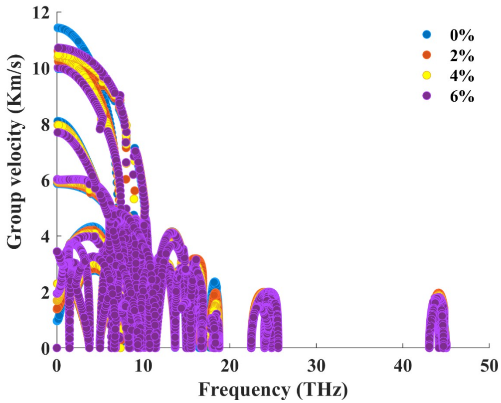
Figure S2: The effect of applied mechanical strain (%) on the phonon group velocity calculated from DLP
