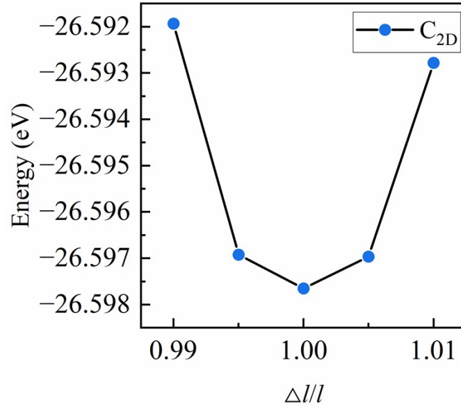
Figure. S1. The total energy as a function of strain in monolayer
