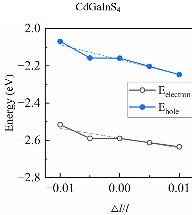
Figure. S2. The band edge energy as a function of strain in monolayer
