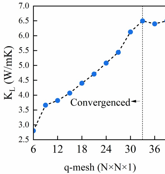
Figure. S3. Convergence test of calculated thermal conductivity for different q-mesh grid.
