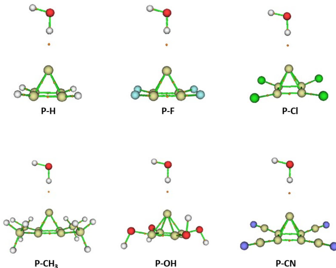
Figure S7. Calculated hydrogen bond critical points for studied systems
