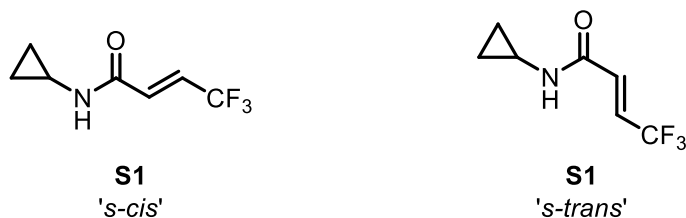
Figure S1. (a) Speciation of the rhodium(I) catalyst reported by Lautens in 2018 and (b) possible substrate conformations.
