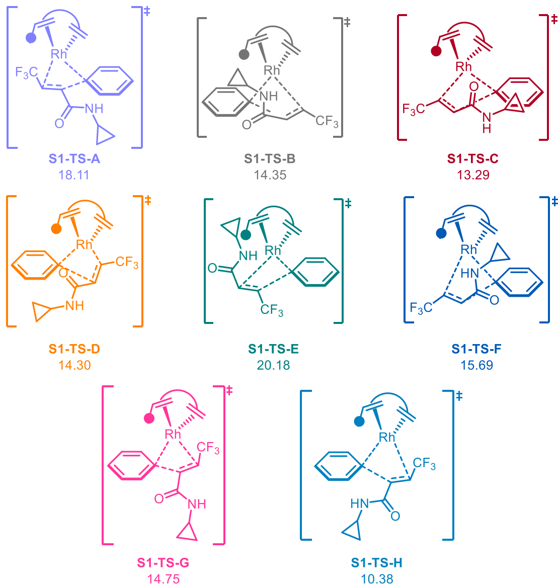
Figure S3. All possible transition states for the migratory insertion step in the defluorinative \alpha -arylation reported by Lautens in 2018.
