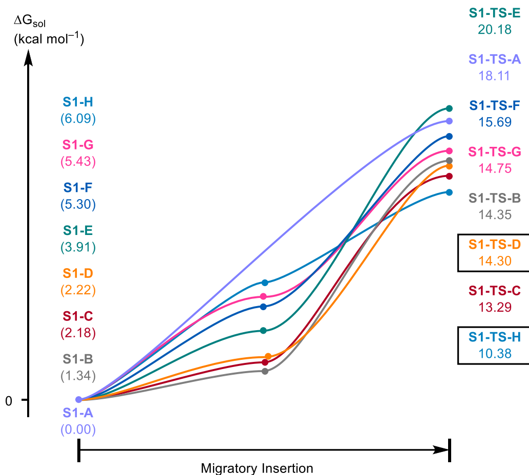
Figure S4. Reaction profile for the regio-reversed migratory insertion of secondary acrylamides. The surface does not include transition states required to undergo rearrangement from S1-A to the other possible conformations.
