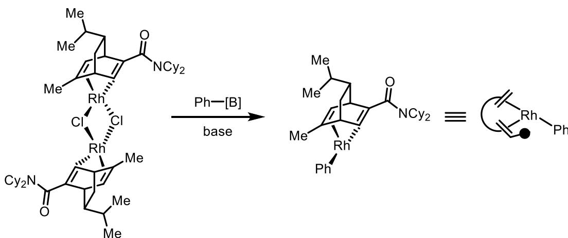
a) Breaking of the C 2 -symmetric rhodium(I) dimer
