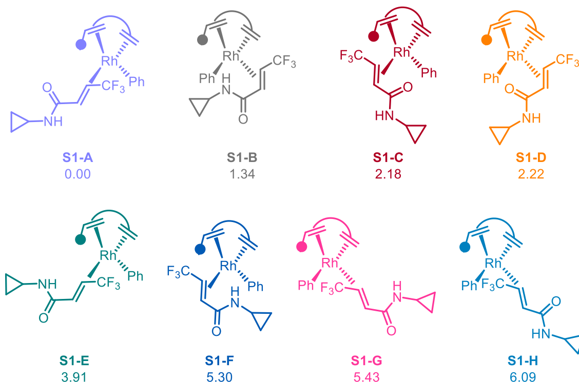
Figure S2. Possible binding modes of the secondary acrylamide to the C 1 -symmetric rhodium catalyst.
