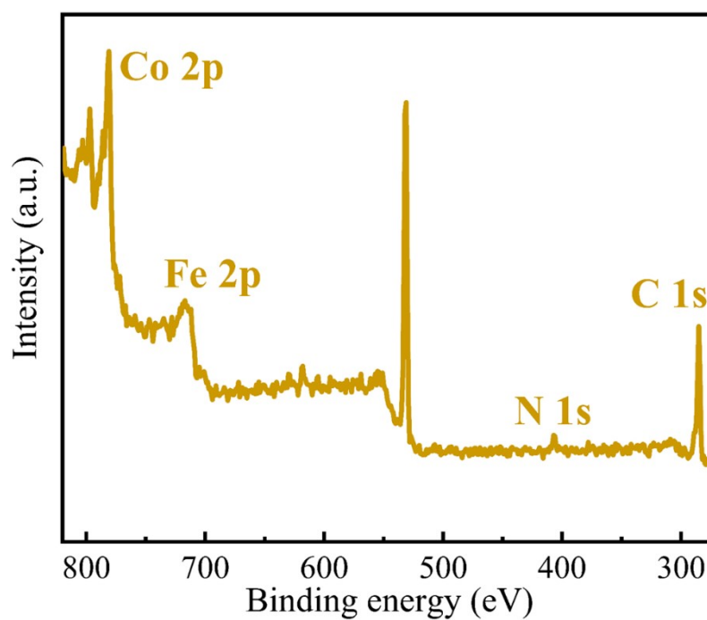
Figure S2. The XPS spectra for CoFe-ZIF.
