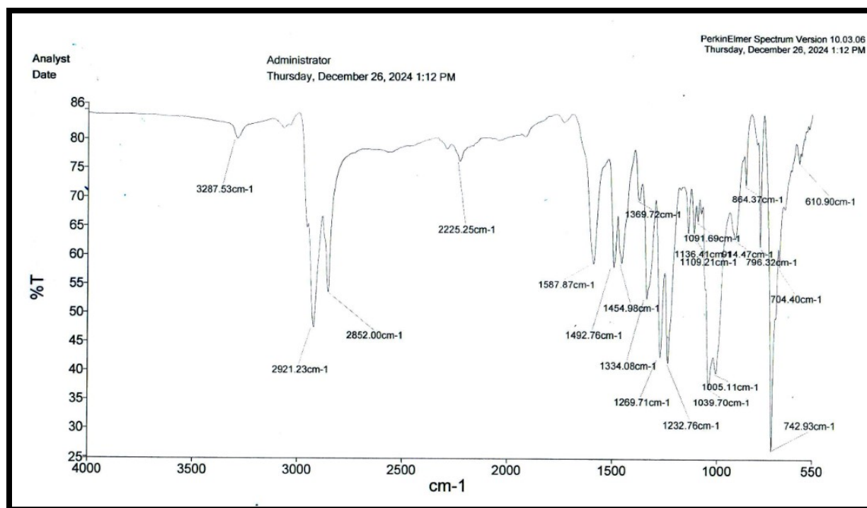
Supplementary Figure 1. FT-IR spectra of synthesized 2(3), 9(10), 16(17), 23(24)-Tetrakis-[dec-2-yn-1-yloxy]phthalocyanine ( H_2Pc ).
