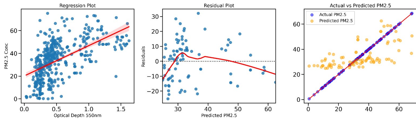
Figure S5. Scatter plot for Airnote PM2.5 concentrations and AOD 550nm for dry season
