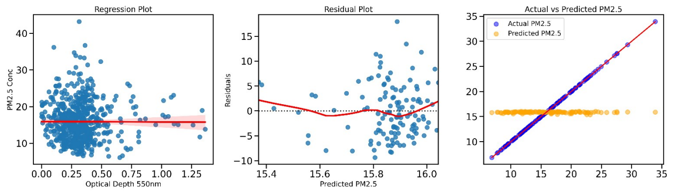
Figure S4. Scatter plot of corrected Clarity PM2.5 concentrations and AOD 550nm for wet season
