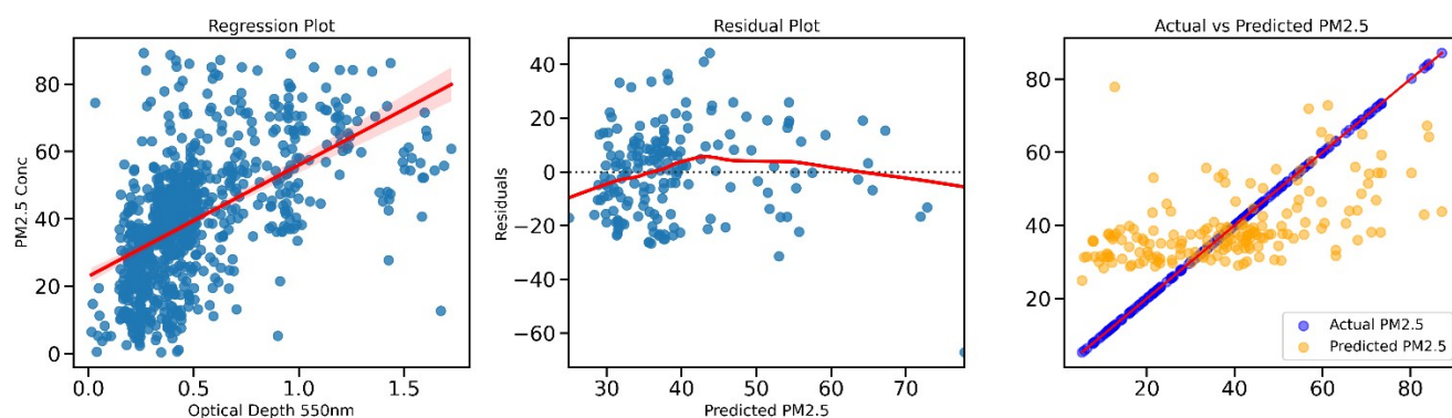
Figure S1. Scatter plot of uncorrected Clarity PM2.5 concentrations and AOD 550nm for dry season
