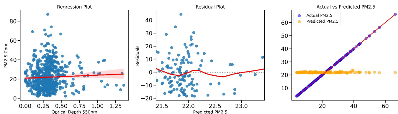
Figure S2. Scatter plot of uncorrected Clarity PM2.5 concentrations and AOD 550nm for wet season
