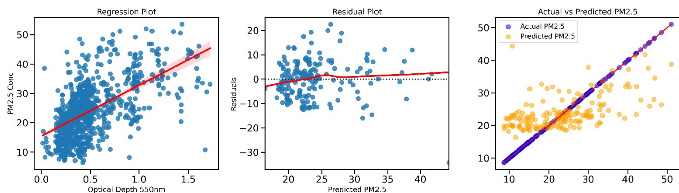
Figure S3. Scatter plot of corrected Clarity PM2.5 concentrations and AOD 550nm for dry season
