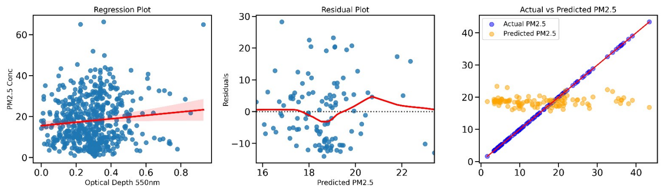
Figure S6. Scatter plot for Airnote PM2.5 concentrations and AOD 550nm for wet season
