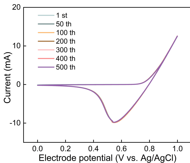
Fig. S18 CV stability test of TiCGC at the scan rate of 50 \text{ mV s}^{-1} in the electrolyte of 2 \text{ M ZnBr}_2 + 3 \text{ M KCl} (vs. Ag/AgCl).
