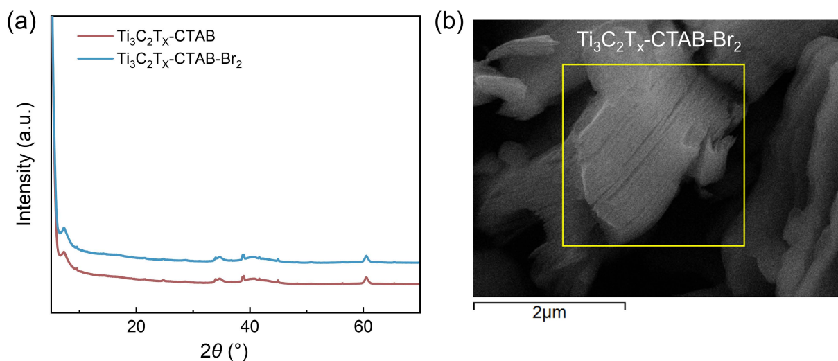
Fig. S19 (a) The XRD patterns of \text{Ti}_3\text{C}_2\text{T}_x\text{-CTAB} and \text{Ti}_3\text{C}_2\text{T}_x\text{-CTAB-Br}_2 (after \text{Ti}_3\text{C}_2\text{T}_x\text{-CTAB} reacting with bromine species). (b) SEM image of \text{Ti}_3\text{C}_2\text{T}_x\text{-CTAB-Br}_2 .
