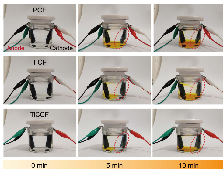
Fig. S23 Photos of the color change during charging in 2 M \text{ZnBr}_2 + 3 M KCl.
