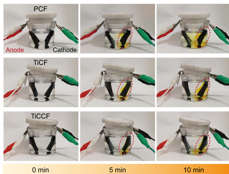
Fig. S24 Photos of the color change during charging in 2 M ZnBr_2 + 3 M KCl + 0.4 M MEPBr.
