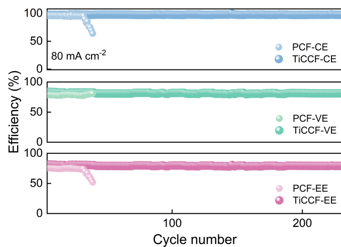
Fig. S25 Cycling performance of the ZBFs using PCF and TiCCF cathodes (electrolytes contained no BCAs) at 80 \text{ mA cm}^{-2} .
