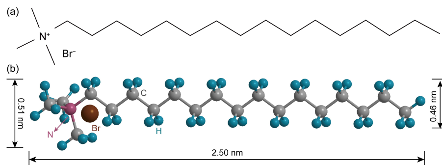
Fig. S1 The formula and 3D structure of CTAB.
