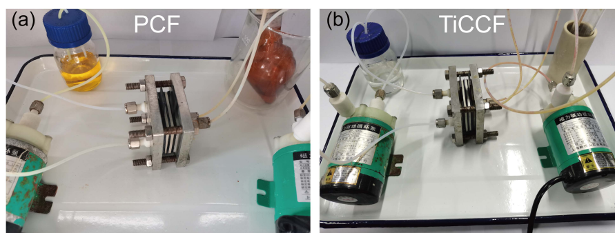
Fig. S26 The electrolyte diffusion phenomenon of the BCA-free ZFBs using (a) PCF and (b) TiCCF as cathodes at 80 \text{ mA cm}^{-2} .
