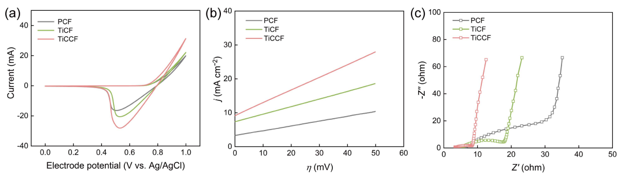
Fig. S28 Electrochemical performance of PCF, TiCF and TiCCF in 2 M ZnBr 2 + 3 M KCl (without BCAs). (a) CV curves at the scan rate of 10 mV s -1 . (b) LSV curves at the scan rate of 1 mV s -1 . (c) Nyquist plots.
