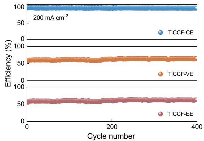
Fig. S29 Cycling performance of the BCA-free ZFBF using TiCCF cathode at 200 mA cm -2 .
