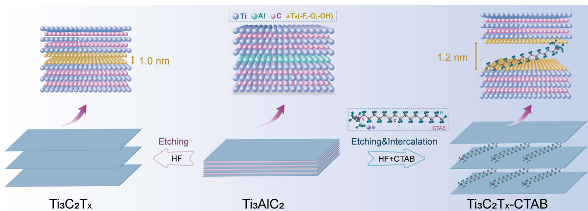
Fig. S3 Schematic illustration for the synthesis of Ti_3C_2T_x MXene and Ti_3C_2T_x-CTAB .
