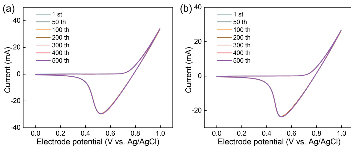
Fig. S30 CV stability test of TiCCF at the scan rate of 50 \text{ mV s}^{-1} in the electrolyte of (a) 2 \text{ M ZnBr}_2 + 3 \text{ M KCl} and (b) 2 \text{ M ZnBr}_2 + 3 \text{ M KCl} + 0.4 \text{ M MEPBr} (vs. Ag/AgCl).
