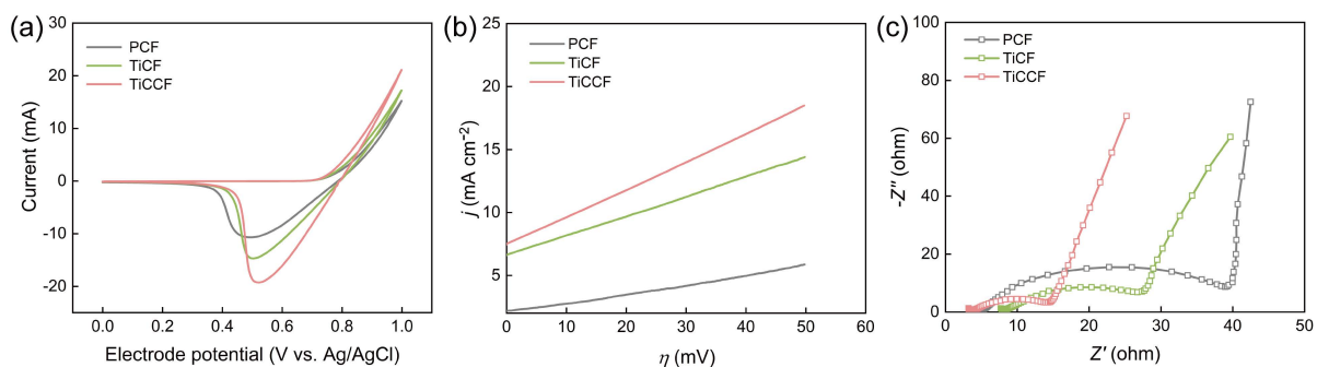
Fig. S31 Electrochemical performance of PCF, TiCF and TiCCF in 2 M ZnBr 2 + 3 M KCl + 0.4 M MEPBr (with BCAs). (a) CV curves at the scan rate of 10 mV s -1 . (b) LSV curves at the scan rate of 1 mV s -1 . (c) Nyquist plots.
