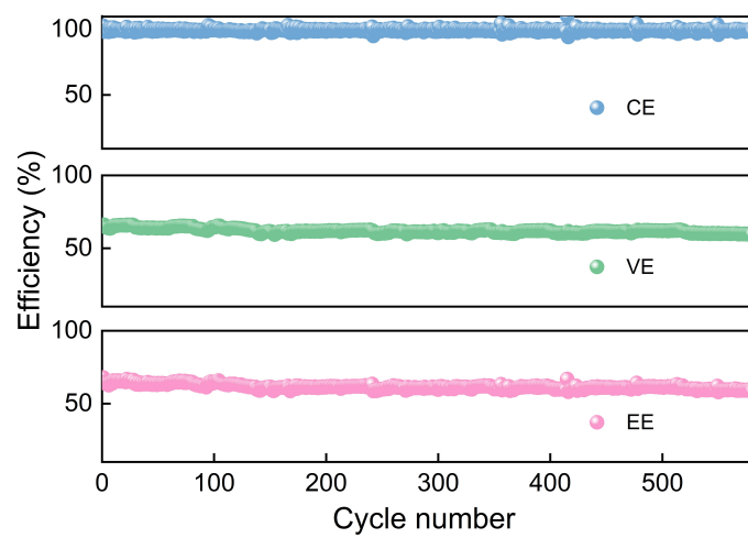
Fig. S33 Cycling performance of the ZFBF using TiCCF cathode at 180 \text{ mA cm}^{-2} .
