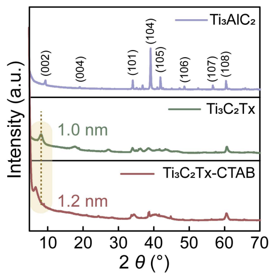
Fig. S5 The XRD patterns of \text{Ti}_3\text{AlC}_2 , \text{Ti}_3\text{C}_2\text{T}_x and \text{Ti}_3\text{C}_2\text{T}_x\text{-CTAB} .
