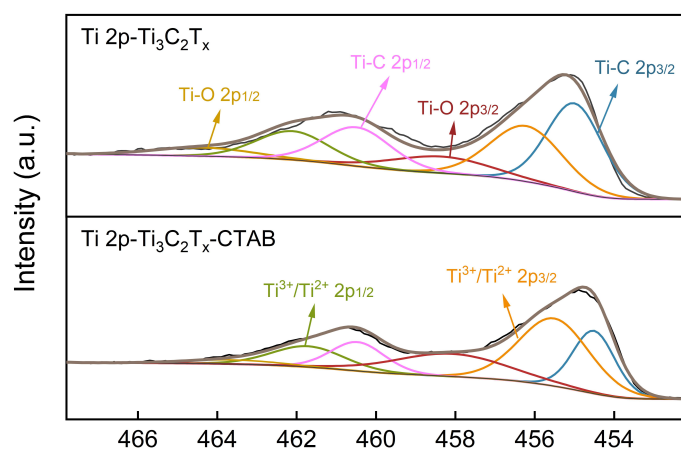
Fig. S8 High-resolution Ti 2p XPS spectra of Ti 3 C 2 T x and Ti 3 C 2 T x -CTAB.
