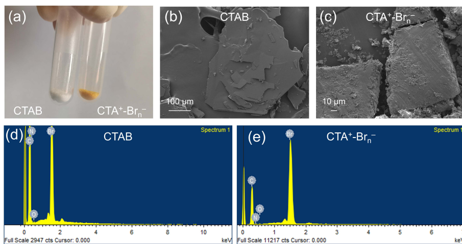
Fig. S11 (a) Photographs of CTAB and CTA + -Br n - . SEM images of (b) CTAB and (c) CTA + -Br n - . EDS energy spectra of (d) CTAB and (e) CTA + -Br n - .
