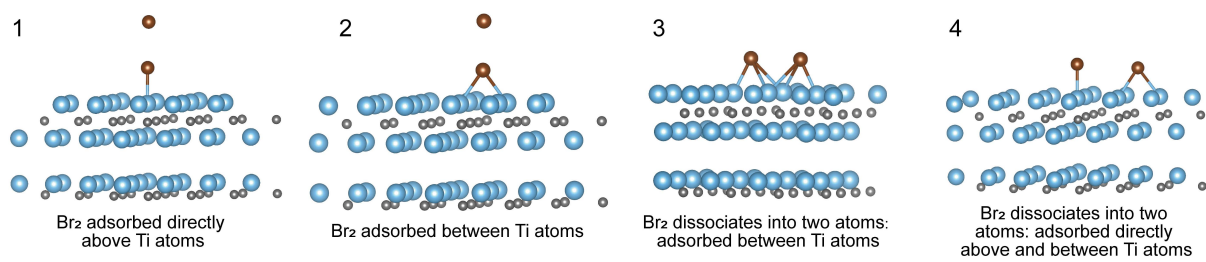
Fig. S15 Four structures of \text{Ti}_3\text{C}_2\text{T}_x surfaces which absorb bromine molecules (blue spheres: Ti atoms; gray spheres: C atoms; brown spheres: Br atoms).
