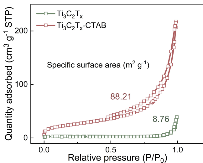
Fig. S16 \text{N}_2 sorption isotherms curves of \text{Ti}_3\text{C}_2\text{T}_x and \text{Ti}_3\text{C}_2\text{T}_x\text{-CTAB} .
