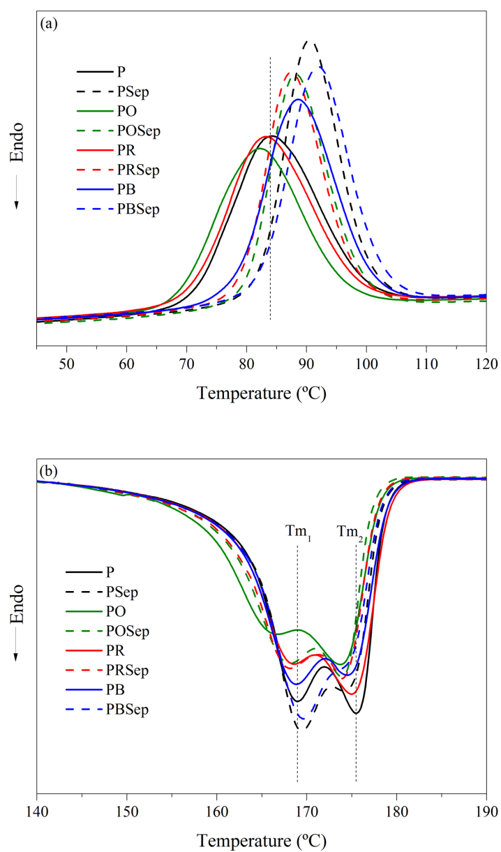
Suppl. Fig. 3. (a) Crystallization and (b) melting DSC curves for pure PHBV and PHBV compositions.
