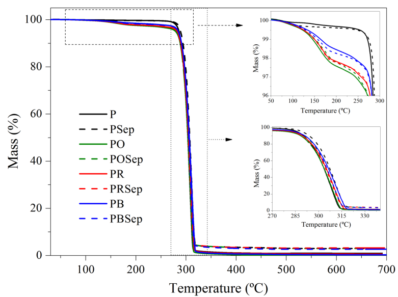
Suppl. Fig. 2. TGA curves for pure PHBV and PHBV compositions.
