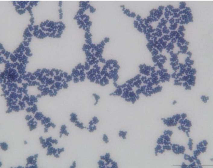
Supplementary figure 1. Gram staining results (A) and neighbor-joining (NJ) phylogenetic tree (B) of KYS-164.
