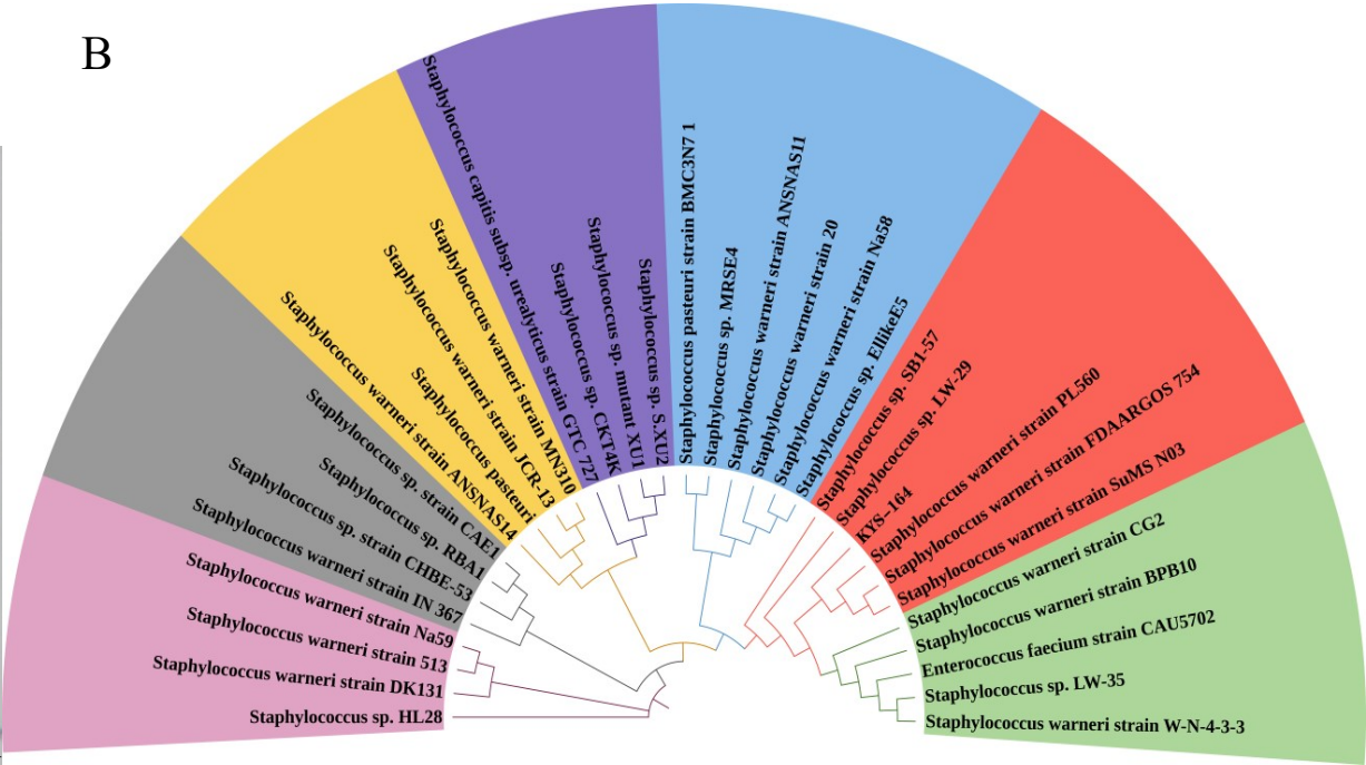
Supplementary figure 1. Gram staining results (A) and neighbor-joining (NJ) phylogenetic tree (B) of KYS-164.
