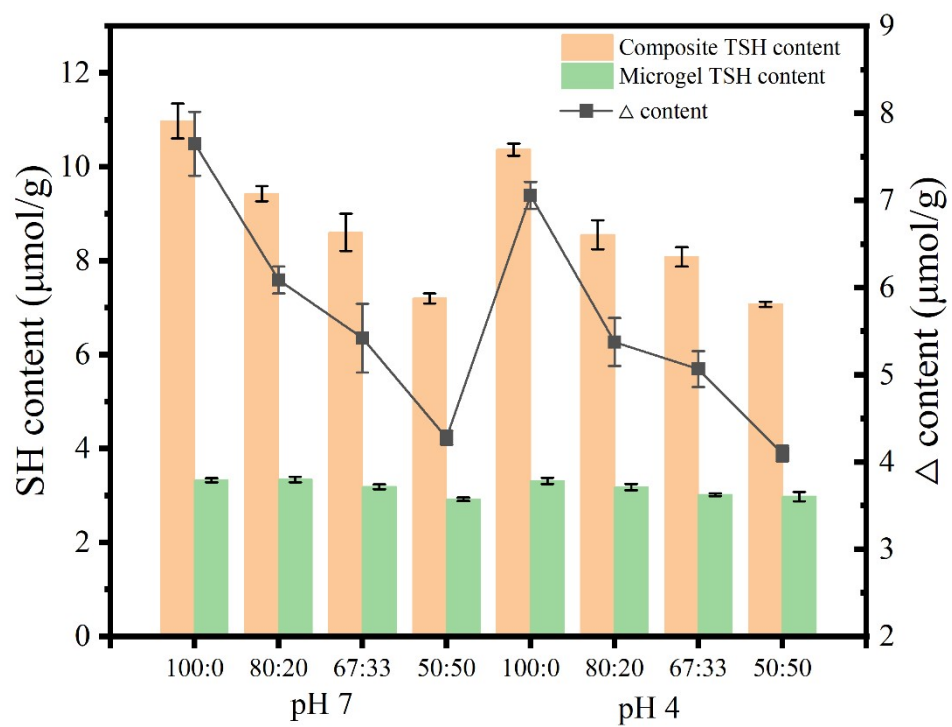
Figure S2. The free sulphydryl content in SPI-EW composites and microgel particles.
