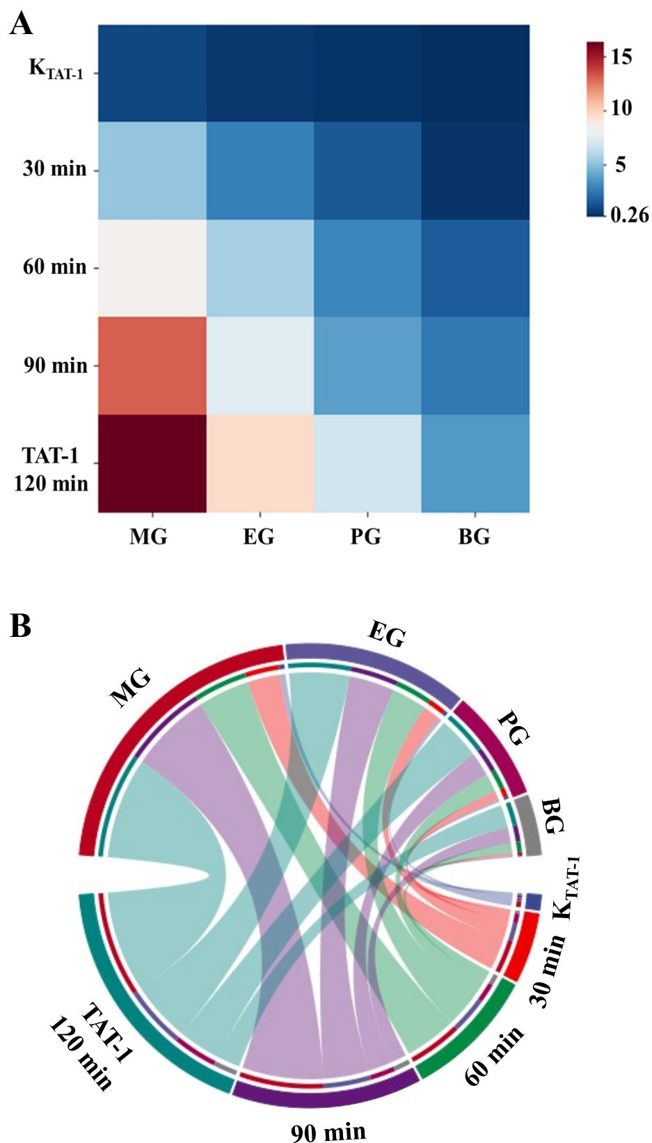
Figure 3S. Heatmap (A) and chord diagram (B) for the transportation of alkyl gallates in everted rat gut sac model. MG, methyl gallate; EG, ethyl gallate; PG, propyl gallate;
