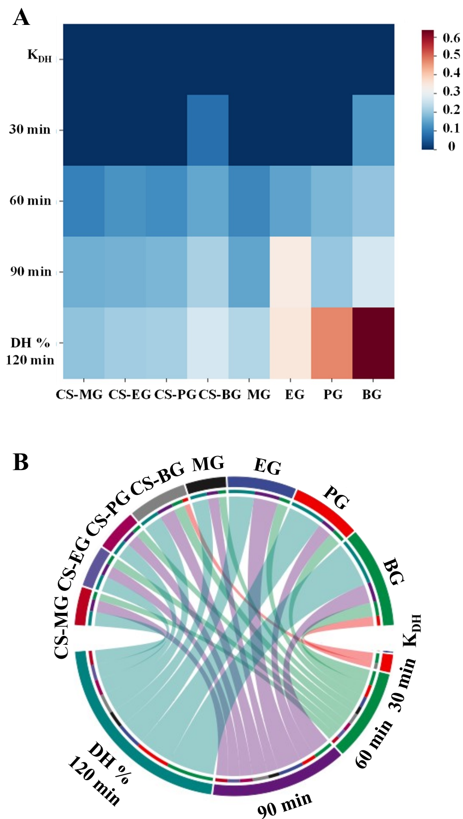
Figure 4S. Heat map (A) and chord diagram (B) for the hydrolysis of alkyl gallates in everted rat gut sac model. MG, methyl gallate; EG, ethyl gallate; PG, propyl gallate; BG, butyl gallate.
