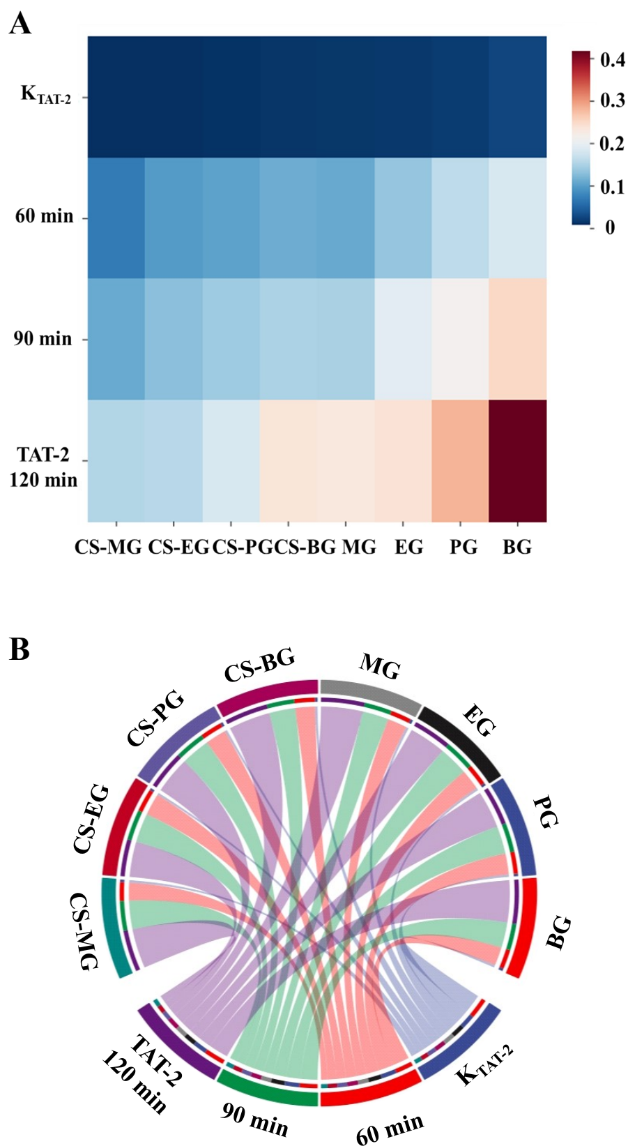
Figure 5S. Heat map (A) and chord diagram (B) for the transportation of gallic acid in everted rat gut sac model. MG, methyl gallate; EG, ethyl gallate; PG, propyl gallate;
