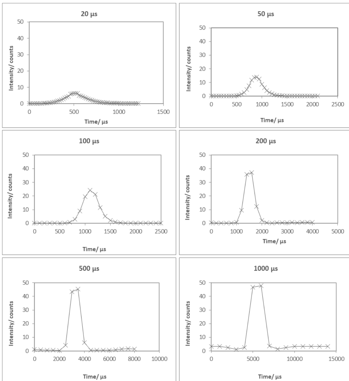
Figure S1: Dwell time optimization from 20 to 1000 \mu\text{s}
