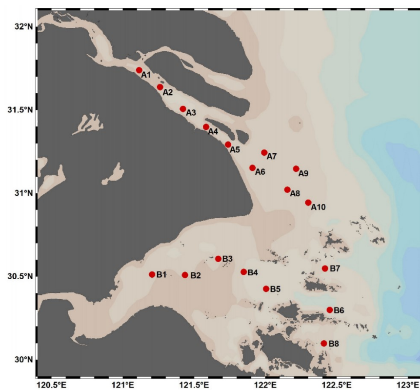
Fig. S1 Sampling stations from the Yangtze River Estuary and Hangzhou Bay from August 24 to 29, 2019.
