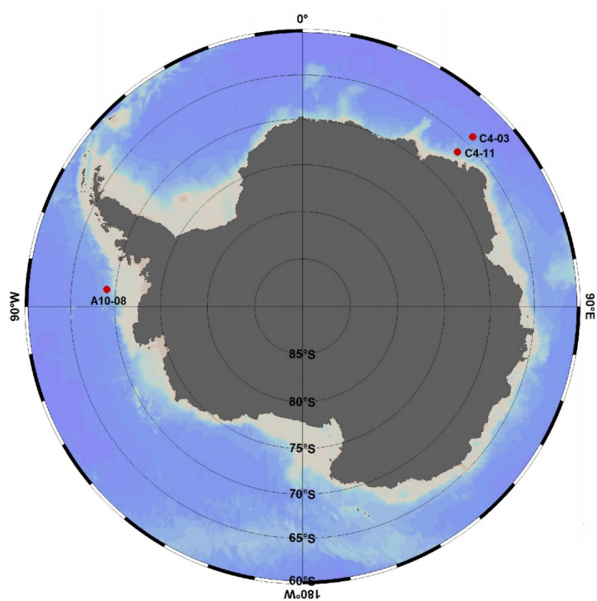
Fig. S3 CTD profiles from the regions around the Antarctic during 37th cruise by Xuelong 2 from November 10, 2020, to May 6, 2021.
