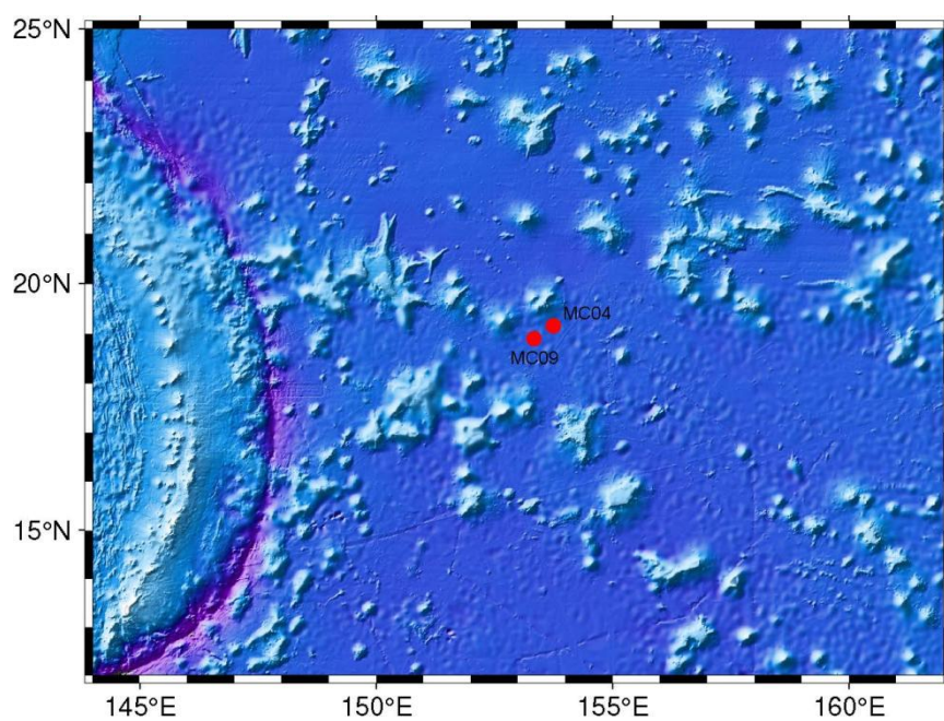
Fig. S2 Multi corer stations from the Pigafetta basin of the West Pacific on October 2023 during the 81thCruise by the Dayanghao.
