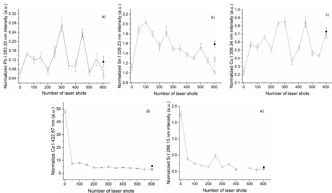
Figure S1 a-e): Depth profiles of normalized LIBS (white squares) and NELIBS (black circles) emission intensity of Pb, Sn, Cu, Ca, and Si in spot C.
