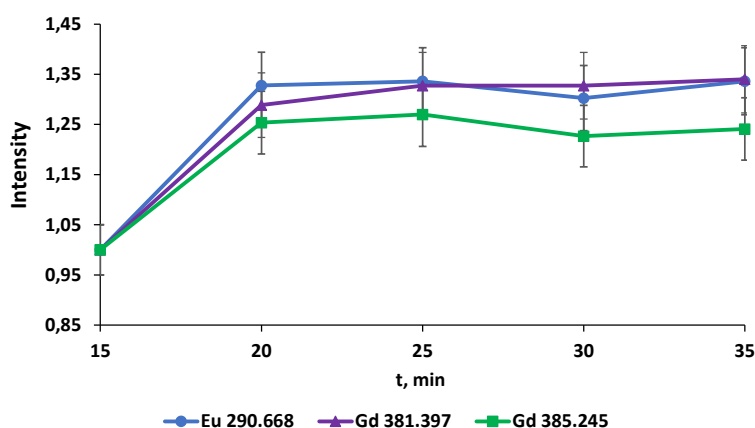
Fig. S1. Dependence of the measured relative intensities of Eu and Gd lines on the spectrometer operation time from the moment of plasma ignition.
