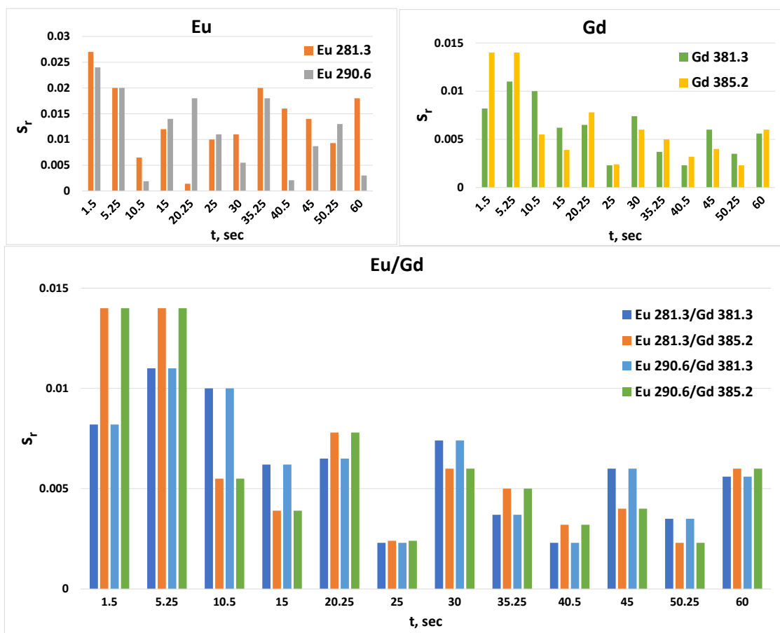
Fig. S2. Dependence of RSDs absolute (top) and relative (bottom) intensities of Eu and Gd lines on the signal registration time.
